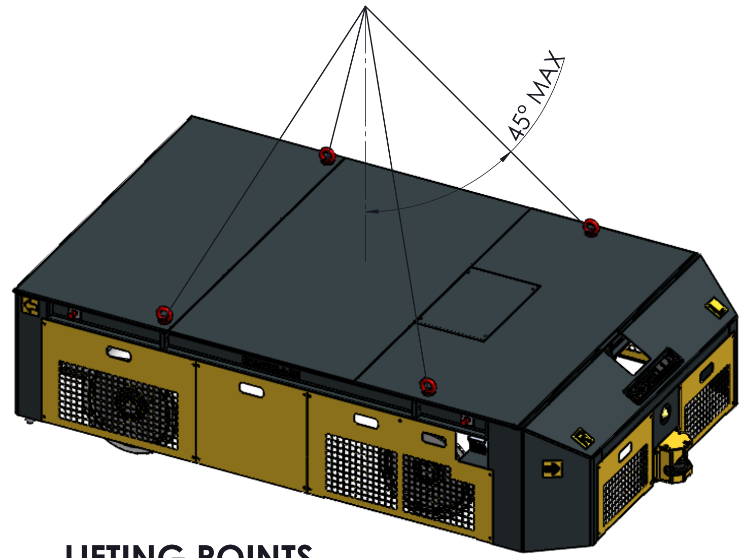
LIFTING POINTS
